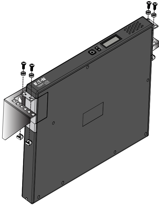
Figure 9. Wallmount
