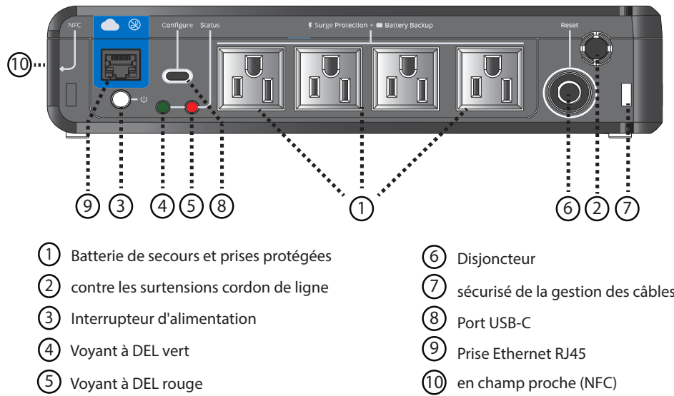
Figure 5. BC850RNC(AG-0761)
