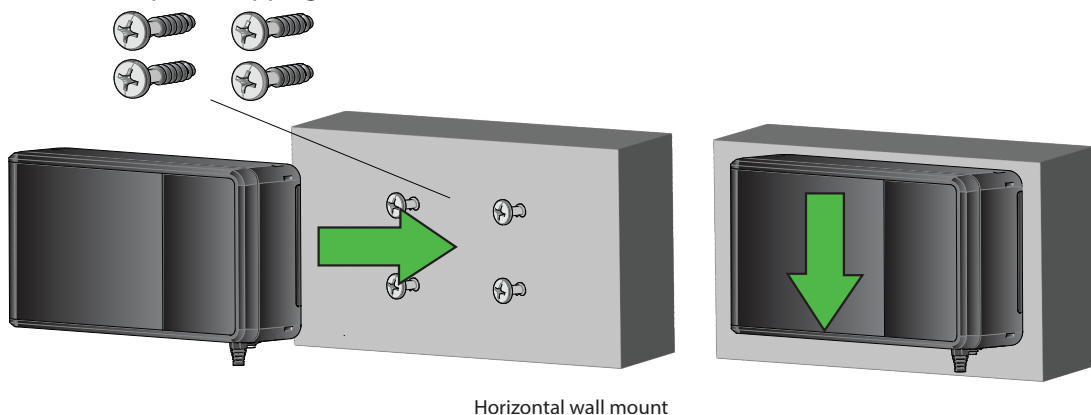
M4x20 Phillips self-tapping screws
