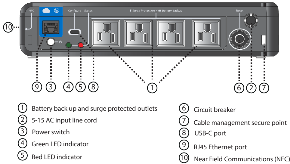
Figure 5. BC850RNC(AG-0761)
