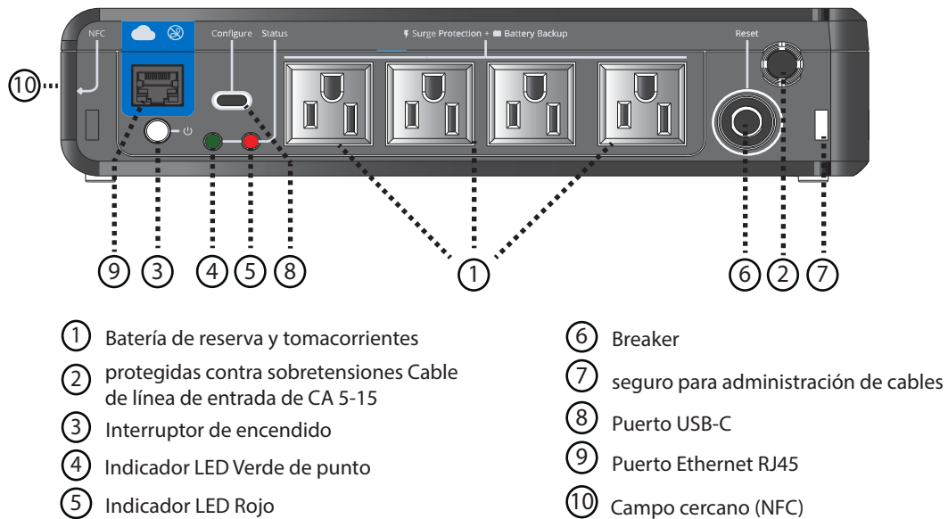
Figure 5. BC850RNC (AG-0761)
