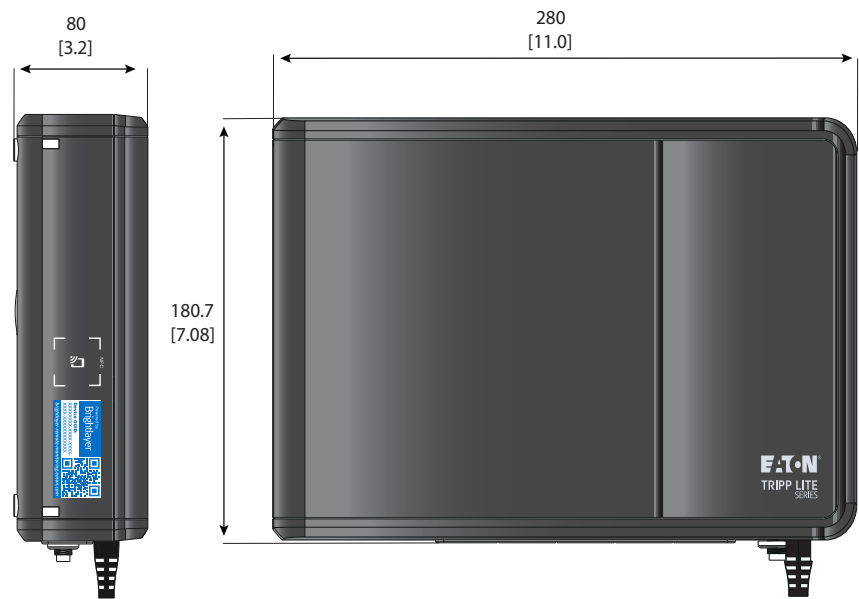
Figure 2. BC850RNC(AG-0761) Dimensions
