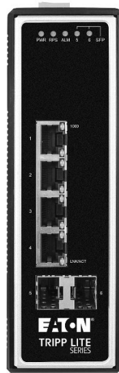
4 10/100/1000Base-T ports & 2 Gigabit SFP slots Managed Industrial Ethernet Switch
